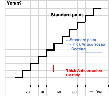
LCC comparison for 100 years of service
